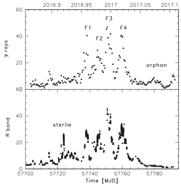
Figure 7. Comparison of the Fermi-LAT \gamma -ray light curve with 12-h time bins (top panel) and R -band light curve (bottom panel) normalized to the lowest value observed in the period 2016 November 11–2017 February 8. Main \gamma -ray outbursts and ‘orphan’ flares are labelled as F1, F2, F3, F4, and orphan in the top panel. The ‘sterile’ flare is labelled as sterile in the bottom panel.
