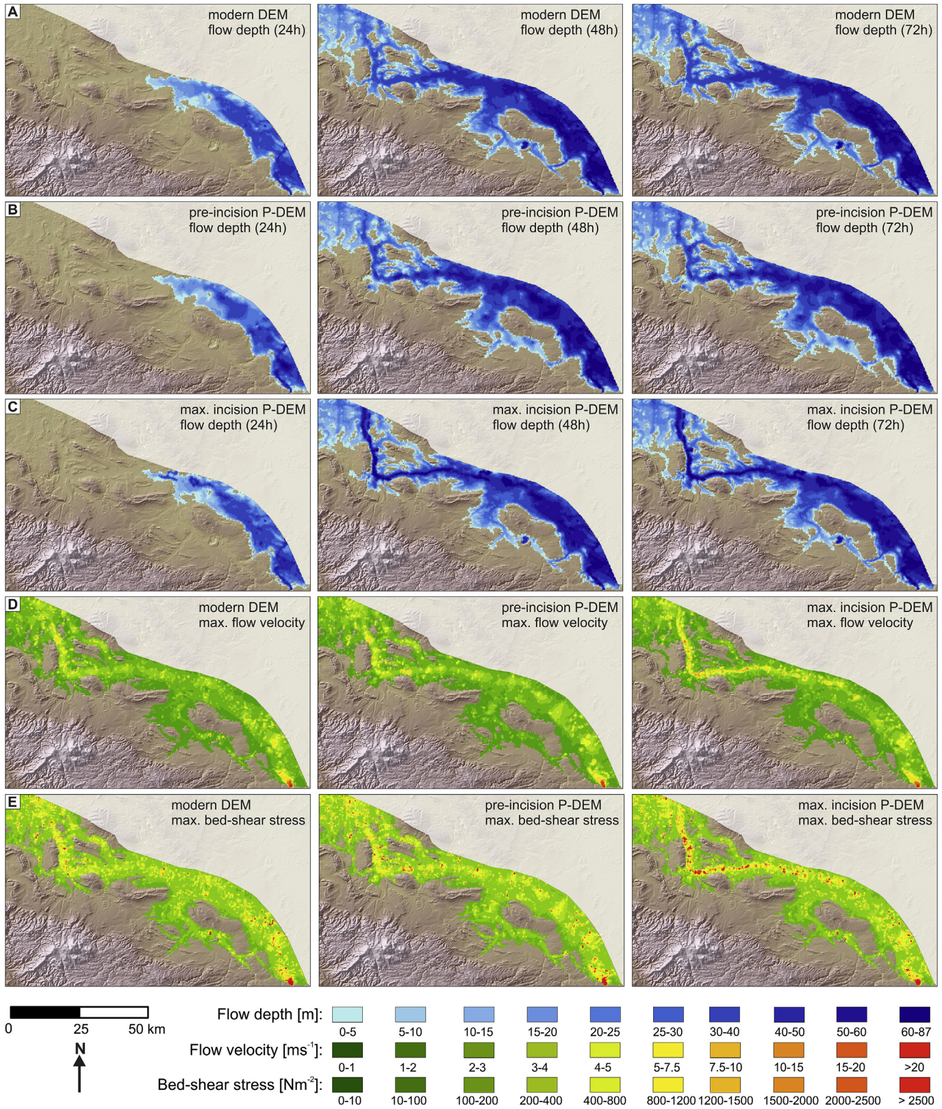
Fig. 10. Comparison of the simulation results. All simulations were run with a hydrograph, where the peak discharge of 502,000 m 3 s -1 is reached after 50 h. A) Flow depth, using the modern topography. B) Flow depth, using the pre-incision palaeotopography. C) Flow depth, using the maximum incision palaeotopography. D) Maximum flow velocity in simulations using the modern topography (left), pre-incision palaeotopography (centre) and maximum incision palaeotopography (right). E) Maximum bed-shear stress in simulations using the modern topography (left), pre-incision palaeotopography (centre) and maximum incision palaeotopography (right).
