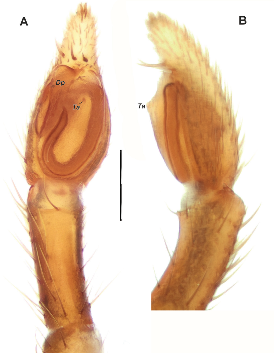
Figure 8. Male palp of Micaria atropatene sp. nov. A ventral B retrolateral. Abbreviations: Dp – distal regular process, Ta – regular apophysis. Scale bar: 0.2 mm.
