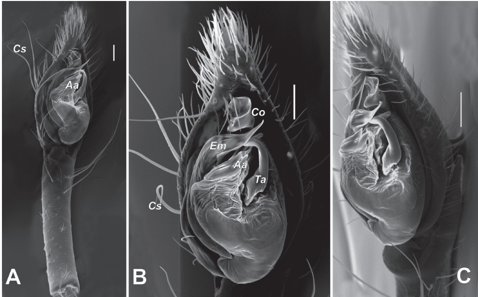
Figure 12. SEM images of the male palp of Mesiotelus patricki sp. nov. A, B ventral C retroventral. Abbreviations: Aa – anterior apophysis, Co – conductor, Cs – curved setae, Em – embolus, Ta – tegular apophysis. Scale bars: 0.1 mm.
