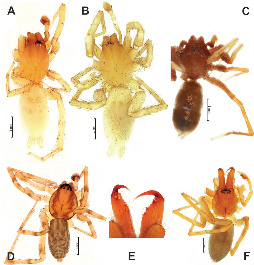
Figure 4. Males of Zagrotes borna sp. nov. (A), Z. parla sp. nov. (B), Micaria atropatene sp. nov. (C), Sestakovaia byrcania sp. nov. (D) and Mesiotelus patricki sp. nov. (E, F) A–D, F habitus, dorsal E chelicerae, ventral. Scale bars: 0.2 mm, unless stated otherwise.
