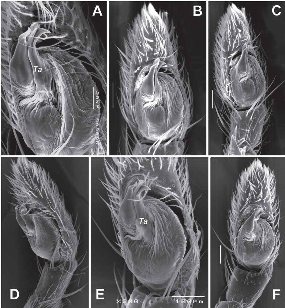
Figure 20. SEM images of the male palp of Rhyssodromus genoensis sp. nov. A, E retroventral B, F ventral C proventral D retrolateral. Abbreviation: Ta – tegular apophysis. Scale bars: 0.1 mm, unless stated otherwise.
