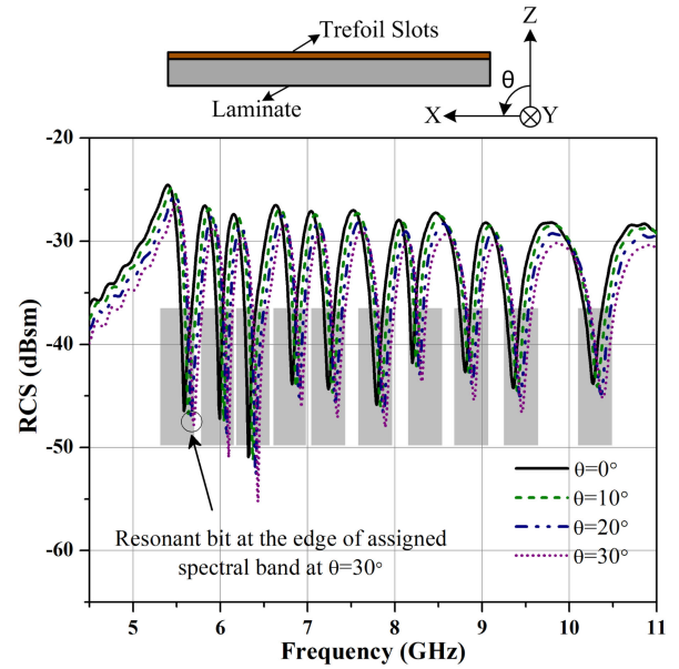
FIGURE 7. Oblique incidence performance for all 1's sequence.
