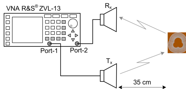
FIGURE 10. Block diagram of tag measurement setup.
