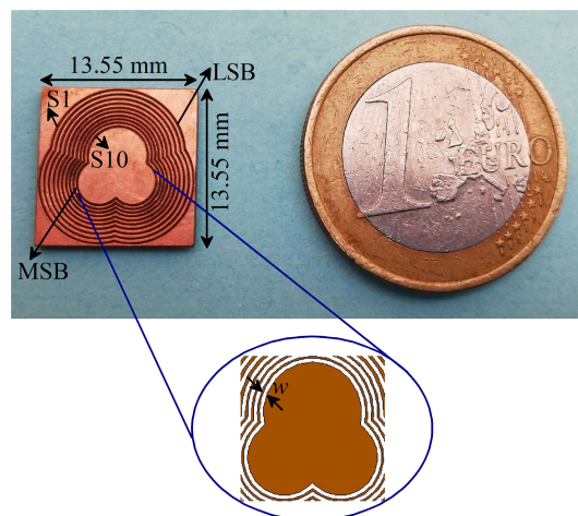
FIGURE 5. Fabricated prototype of 10 bit proposed tag.
