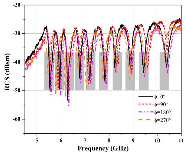
FIGURE 14. Measured RCS response of the tag at different polarization angles.
