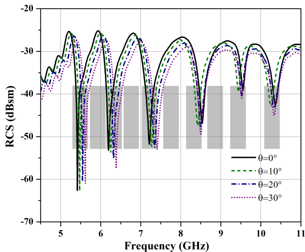
FIGURE 8. Oblique incidence performance for 101010111 sequence.
