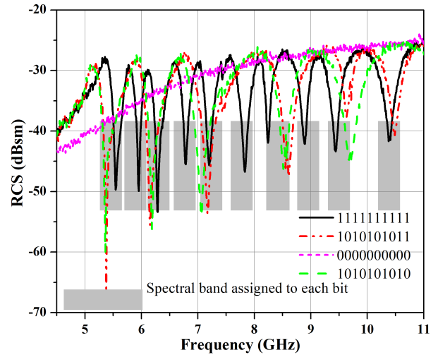
FIGURE 13. Measured RCS response for different bit sequences.
