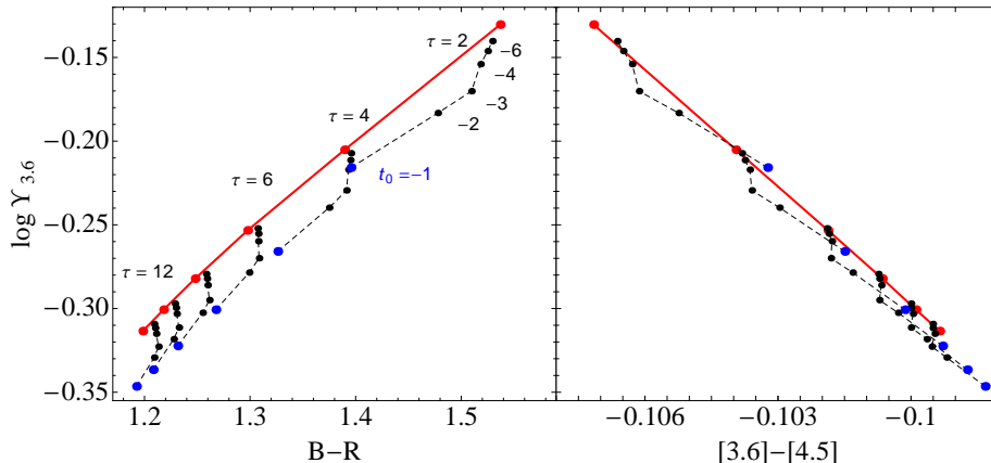
FIG. 3.— Mass-to-light ratio \Upsilon_{3.6} (in solar units M_{\odot}/L_{\odot} ) as a function of B-R and [3.6]-[4.5] color for a sequence of exponentially declining star formation rate models at solar metallicity ( Z=0.02 ) with 10% mass fraction added in 0.5 Gyr-duration starbursts. The solid red line connects the exponential SFH models with different e-folding timescales \tau from Figure 2. The dashed lines connect models of the same \tau with starbursts occurring 1, 2, 3, 4, or 6 Gyr ago. The SFH with the youngest mean age (latest burst) is shown in blue for each underlying decaying exponential.
