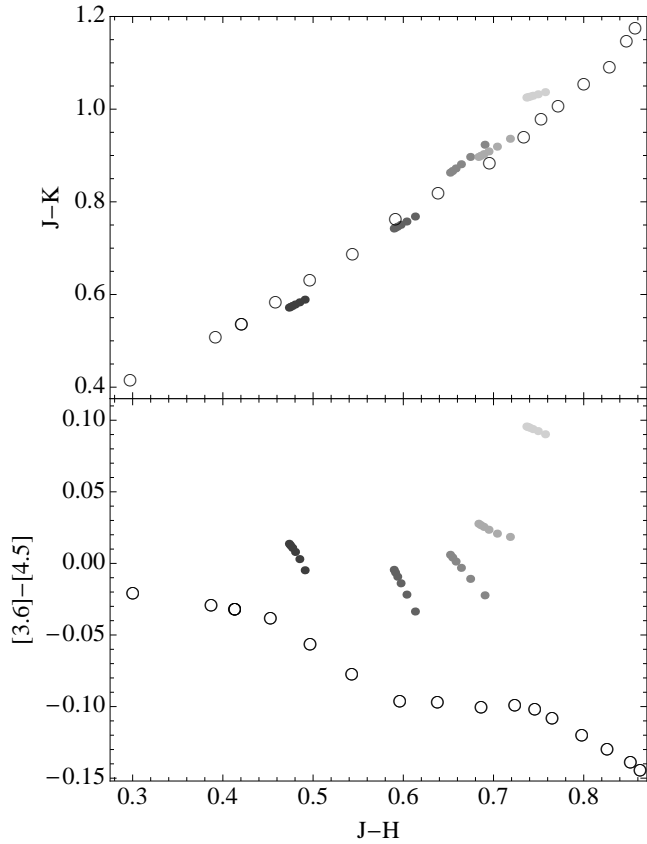
FIG. A2.— Comparison between the NIR colors of giant stars (open circles) and BC03 SPS models (filled circles) considered in Figures 1 and 2. The gray scaling of the model points varies with SPS metallicity from low (black) to high (light gray). At each metallicity, a range of ages is shown (see Figure 2).
