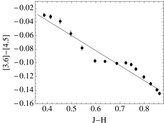
FIG. A1.— The mean [3.6]-[4.5] color and its error for each of the 15 spectral classes against the J-H color of each class of giants. Each bin contains hundreds of stars. The solid black line shows our best-fit linear relation between the [3.6]-[4.5] and J-H colors of GLIMPSE giants sorted by spectral type. (Table A1).
