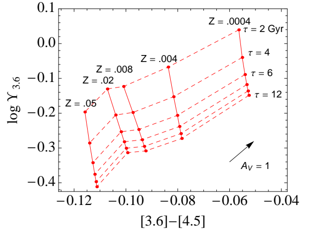
FIG. 2.— \Upsilon_{3.6} - ([3.6]-[4.5]) relation for a sequence of exponentially declining star formation rate models from Figure 1, using the calibration between J-H and [3.6]-[4.5] in Appendix 1 to link the BC03 models to [3.6]-[4.5] color. Models of the same e-folding timescale \tau are connected by dashed lines, while models of the same metallicity Z are connected by solid lines. The black arrow in the bottom right corresponds to V-band extinction A_V=1 , assuming a Galactic extinction law (Cardelli et al. 1989; Indebetouw et al. 2005).
