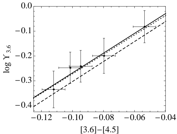
FIG. 4.— Relation between fixed-metallicity bins of \Upsilon_{3.6} and [3.6]-[4.5] measured from the sequence of exponentially declining star formation rate models shown in Figure 2, with errors as described in the text. The solid black line shows our best-fit relation. The dashed and dotted lines show the results of fits over a restricted range of metallicity and age (see Table 1). The bluest point ( Z=0.0004 ) has been omitted for the fit traced by the dotted line, while the dashed line shows the fit to slightly different bins (not shown) from which the model with the oldest age at each metallicity is omitted.
