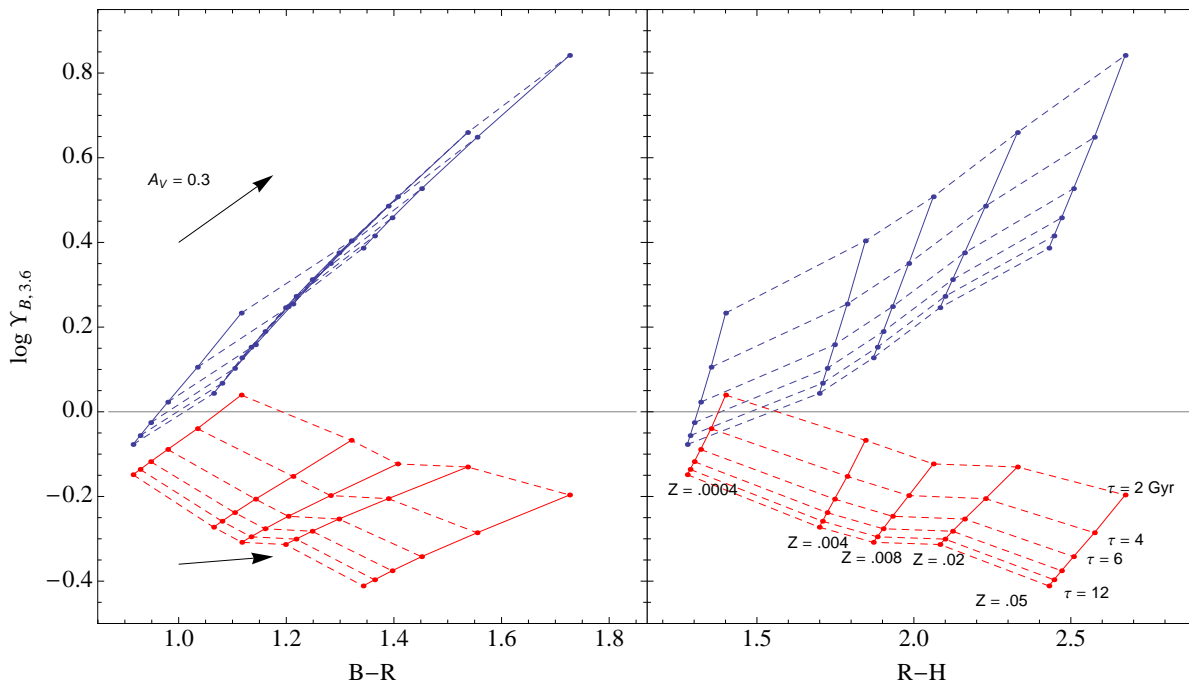
FIG. 1.— Trends in stellar M/L ratios (in solar units M_{\odot}/L_{\odot} ) with optical and optical-NIR color for simple exponential SFH models of age 13 Gyr from BC03. The blue lines (top grid) show B-band \Upsilon_B , and the red lines (bottom grid) show 3.6 \mu\text{m} \Upsilon_{3.6} . Models of the same e-folding timescale \tau are connected by dashed lines, while models of the same metallicity Z are connected by solid lines. Short (long) \tau correspond to older (younger) ages. The black arrows in the top and bottom of the left panel corresponds to V-band extinction A_V=0.3 , assuming a Galactic extinction law (Cardelli et al. 1989; Indebetouw et al. 2005).
