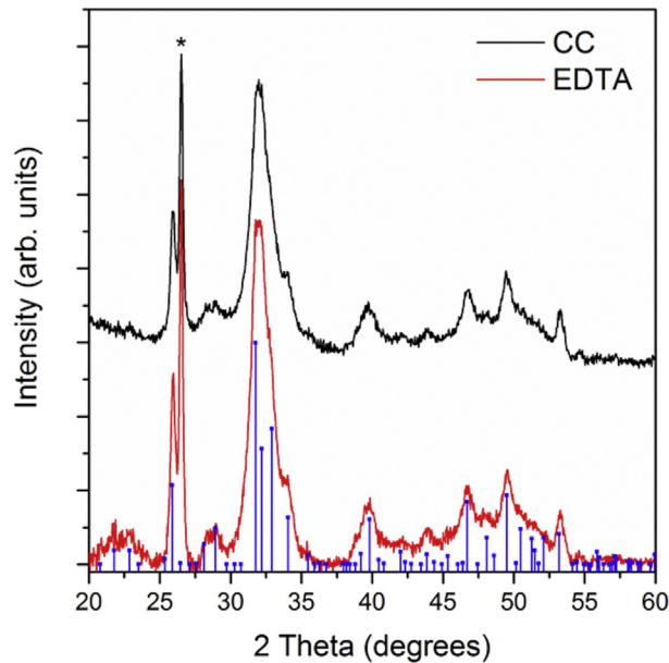
Fig. 5. XRD diffractograms of functionalized calcium carbonate samples (CC shown in black) and EDTA (red). The asterisk (*) indicates an impurity phase of graphite after carbon sputtering.
