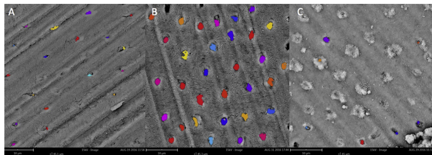
Fig. 2. Scanning electron microscopy (SEM) images of dentine surfaces and porometric analysis of A. cut surface with smear layer; B. EDTA treated; C. FCC grit blasted samples. Colored areas represent the open tubules. Original magnification \times 6000 , bar = 10 \mu\text{m} .
