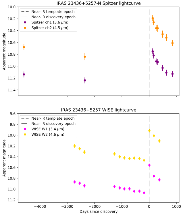
Figure 4. Top panel shows the Spitzer lightcurve at 3.6\ \mu\text{m} and 4.5\ \mu\text{m} of the Northern nucleus of IRAS 23436+5257. Bottom panel shows the archival WISE lightcurve at 3.4\ \mu\text{m} and 4.6\ \mu\text{m} of the full host galaxy. In the Spitzer data the host nucleus of AT 2017gbl is resolved, whereas in the WISE data the host galaxy is not resolved. The vertical lines indicate the epochs of the near-IR reference data set (relevant for the construction of the SED of the transient, see Section 3.3.1) and the near-IR discovery epoch, respectively.
