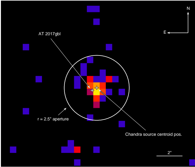
Figure 8. X-ray image of AT 2017gbl obtained with Chandra in 0.5-7 keV band. The circle represents a 2.5'' aperture centered on the X-ray source containing \sim 95\% of emission from the on-axis source, which was used to extract the spectrum shown in Fig. 9. The position of the centroid and the position of AT 2017gbl as observed in the near-IR are also indicated.
