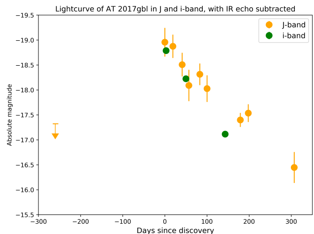
Figure 19. Evolution of AT 2017gbl in i and J after subtraction of the IR component, in absolute magnitudes. The magnitudes are dereddened for a line of sight extinction of A_V = 2.5 mag as determined through Paschen line ratios in Section 3.2.1, and corrected for the Milky Way extinction. Both filters show a similar continuous decline, from which we conclude the IR echo subtracted J -band flux traces the evolution timescale of the optical blackbody component well. The J -band upper limit at epoch -260 days from 2016 October 21 is the latest pre-outburst epoch available to constrain the evolution of the optical component.
