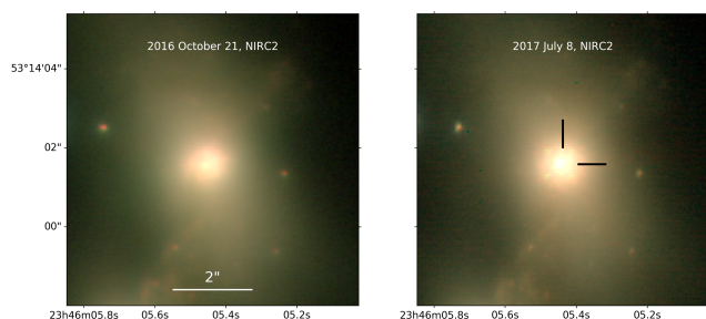
Figure 1. AT 2017gbl coincident with the Northern nucleus of IRAS 23436+5257, discovered with NIRC2. Left panel shows a JHK_s colour composite from the NIRC2 template epoch in October 2016. Right panel shows a JHK_s colour-composite of the discovery epoch of AT 2017gbl in July 2017. Image cutouts are \sim 7.5'' across.
