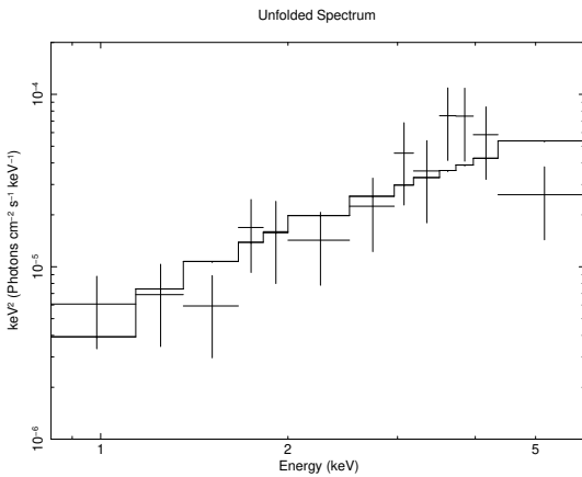
Figure 9. Chandra X-ray spectrum of the source fitted with an absorbed power-law where N_{\text{H}} = 3.0 \times 10^{21} \text{ cm}^{-2} and the fitted photon index is \sim 0.9 .
