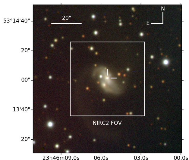
Figure 2. A gri -colour composite image of IRAS 23436+5257 as observed with ACAM on the WHT on 2017 July 10, three days after the discovery of AT 2017gbl. The transient was coincident with the Northern nucleus, indicated by tick marks. The FOV of the Keck NIRC2 discovery image is also shown. The ACAM image cutout shown here is 100'' across.
