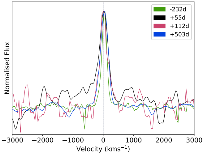
Figure 14. Comparison of the Bry emission line evolution over time. The spectral peaks have been normalised to one after subtraction of a linear fit to the continuum. The only spectrum that shows evidence for a broad component is at +55 days (black line).
