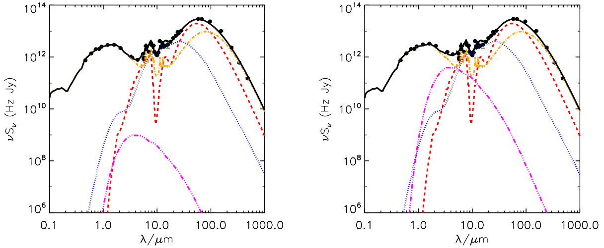
Figure 10. The best fitting SED model for IRAS 23436+5257 obtained using the MCMC code SATMC (Johnson et al. 2013), pre-outburst on the left and post-outburst (+10 days) on the right with the contribution from AT 2017gbl included at the wavelength range 0.5 - 4.6 \mu\text{m} . The flux measurements are indicated by the black dots, and the model SED is composed of a starburst (red), an AGN torus (blue), a spheroidal host (orange) and a polar dust at 1300K (magenta) component.
