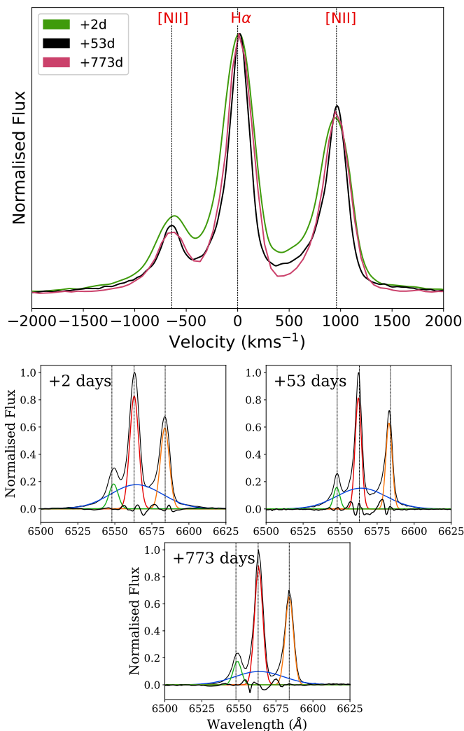
Figure 15. Upper panel: Comparison of the H\alpha region in our optical spectra. The peak of the H\alpha line was normalised to one, after subtraction of a linear background. The earliest spectrum has a stronger contribution from the broad component than the two later observations. Lower panel: Multi-component fitting of the features in the H\alpha region. Data is shown in black, and fit residuals are shown along the x axis.
