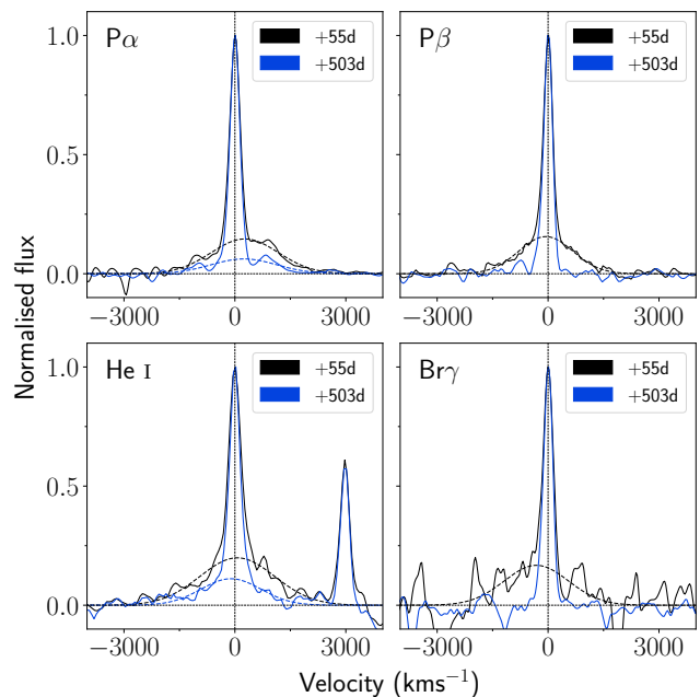
Figure 13. Fits to the emission lines that show more prominent broad features in our GNIRS spectra. The peak of the narrow feature is normalised to 1. Dashed lines show the broad Gaussians that were fitted to the spectra to derive the values listed in Table 2.
