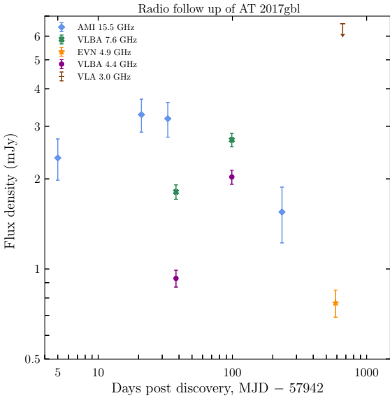
Figure 7. Radio lightcurve of AT 2017gbl. The flux densities from AMI and the VLA have been corrected for host galaxy contributions. The AMI epochs of +848 and +936 days are not shown here, as they are considered transient-free and act as the quiescent level of the host galaxy at 15.5 GHz (see text for details). The epoch at 3 GHz with the VLA has a large uncertainty, and we show the 3\sigma upper limit here instead of the host-subtracted value.
