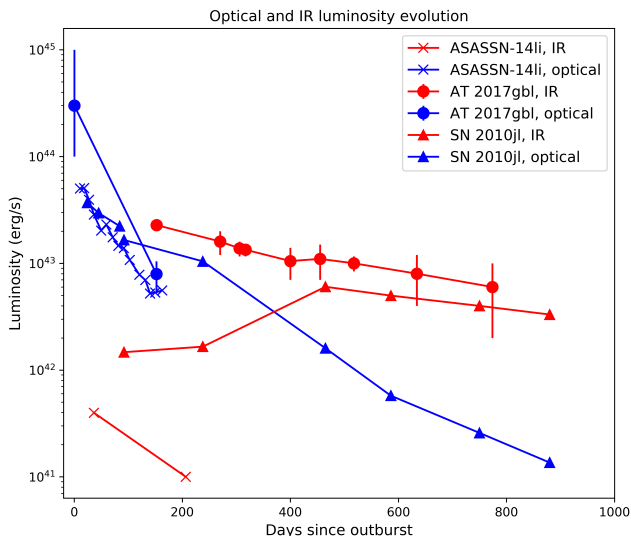
Figure 21. Evolution of the blackbody luminosities of the optical and IR components of AT 2017gbl, SN 2010jl (Zhang et al. 2012; Fransson et al. 2014), and ASASSN-14li (Holoien et al. 2016; Jiang et al. 2016). The first three optical epochs of SN 2010jl are based on bolometric luminosities from Zhang et al. (2012), which should be close to its optical blackbody luminosity because the IR component was negligible at early times. The x-axis start at the outburst epoch (-142 days) of AT 2017gbl inferred in Section 3.3.3, the explosion epoch (MJD 55478) of SN 2010jl (Fransson et al. 2014), and the discovery epoch (MJD 56983) of ASASSN-14li (Holoien et al. 2016). The optical luminosity of AT 2017gbl at day 0 is the range inferred from fitting the blackbody temperature evolution in Section 3.3.3.
