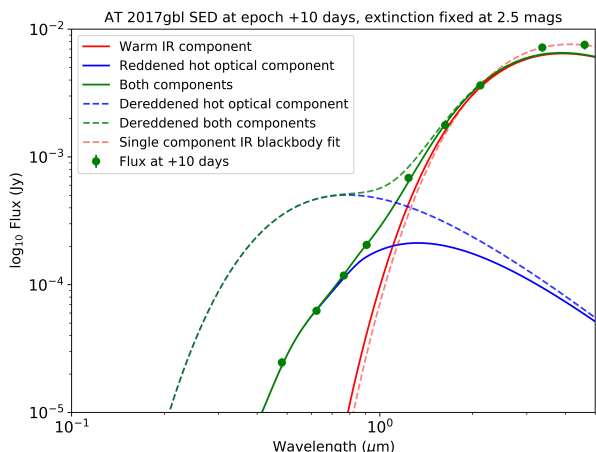
Figure 18. MCMC two components fit to all optical, near-IR and mid-IR fluxes of the epoch +10 days after discovery, with a fixed extinction at A_V = 2.5 mag affecting the optical blackbody. In red is shown the warm IR component, in blue the dust-extincted optical component and in green the sum of the blackbodies and the observed fluxes. The dashed lines indicate the de-reddened intrinsic optical blackbody in blue, and in red the single component fit of the IR blackbody.
