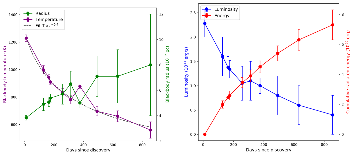
Figure 17. Left panel: evolution of the IR blackbody parameters. Right panel: IR blackbody luminosity and the cumulative radiated energy.
