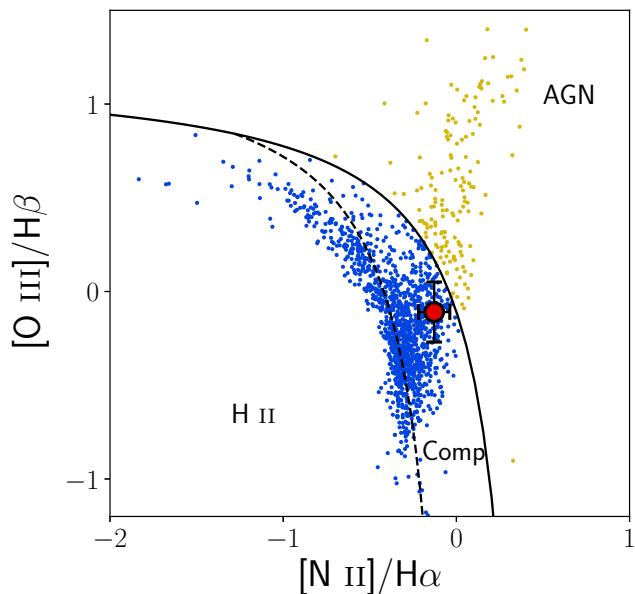
Figure 12. BPT diagram showing the position of IRAS 23436+5257 with a red point. The galaxy data shown is taken from SDSS DR7 (Abazajian et al. 2009), regions indicated are taken from Kewley et al. (2006). Colouring of points indicates the region they lie within, not an independent determination of their type. Code distributed as part of ASTROML (Vanderplas et al. 2012) was adapted to generate this plot.
