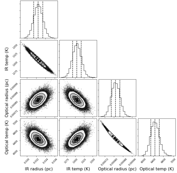
Figure A1. Corner plot of the posterior distributions of the MCMC two components fit to all optical, near-IR and mid-IR fluxes of the epoch at +10 days, see Fig 18. The fitted values are indicated by the center lines, with the 1\sigma confidence interval indicated on either side.
