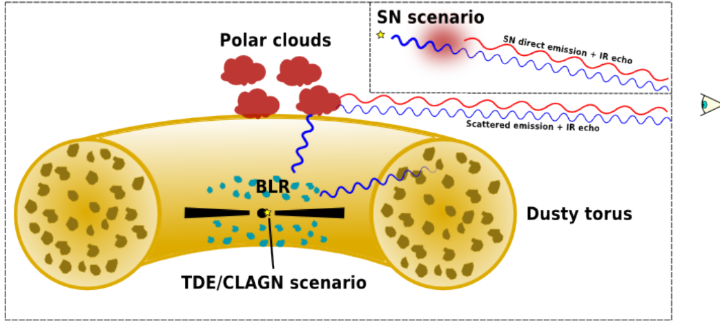
Figure 20. A schematic diagram showing the sources of IR and optical emission (and absorption) in the scenarios for AT 2017gbl either as a SN, or a TDE/CLAGN. Note the components are not to scale. In all scenarios the IR emission is interpreted as an IR echo, where UV/optical emission from the transient is absorbed and re-radiated at IR wavelengths. The optical emission in the case of a SN is considered direct dust-attenuated emission, whereas in the case of a TDE/CLAGN it is considered scattered light originating in the BLR. Direct emission from a TDE/CLAGN is not visible due to the presence of the dusty torus along the line of sight. It must be noted that the potential SN location is not constrained, however, there is 2.5 mag of extinction along the line of sight.
