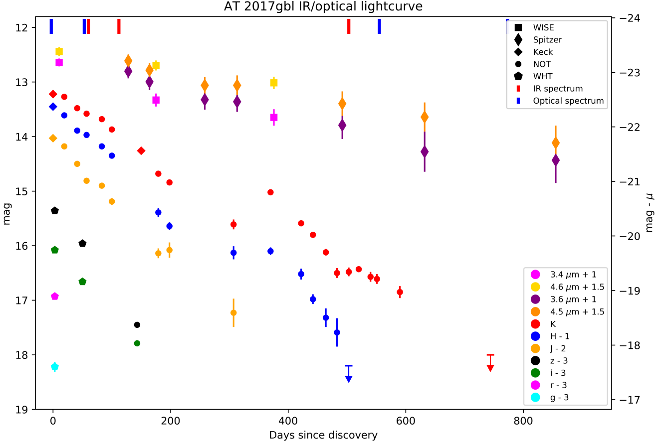
Figure 3. IR and optical evolution of AT 2017gbl. For clarity, the lightcurves have been offset as indicated in the figure legend. IR magnitudes are in the Vega system, optical magnitudes in the AB system. Pre-discovery non-detections are not shown, and consist of a JHK_s near-IR epoch at -260 days, and a 3.4/4.6 \mu\text{m} WISE epoch at -188 days.
