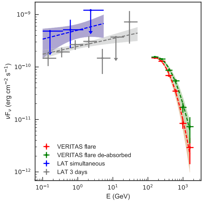
Figure 3. The gamma-ray SEDs of BL Lacertae measured by Fermi -LAT and VERITAS. The Fermi -LAT SEDs that are strictly simultaneous with VERITAS observations on the night of the flare (2016 October 5) and from the three days around it are shown in blue and gray, respectively. The observed and de-absorbed VERITAS SEDs averaged over all observations on the night of the flare are shown in red and green, respectively. Each shaded region is derived from the 1\sigma confidence intervals of the best-fit parameters for the corresponding spectrum.
