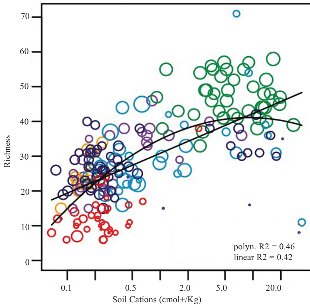
Figure 2. Trends in species richness (i.e. the number of species) of pteridophytes in 214 transects of 500 m x 5 min Amazonian non-inundated forests as a function of measured concentration of exchangeable base cations in the soil. Colours refer to geographical regions: green, Ecuador; orange, Colombia; red, central Amazonia; dark blue, NW Peruvian Amazonia; purple, NE Peru; mid blue, central Peru; light blue, S Peru. The most distant sites are more than 2000 km apart. Symbols are sized in relation to annual rainfall (extracted from WorldClim v. 1.4), which is only weakly correlated with soil cation concentration ( r = 0.21 ). Reprinted, with permission, from figure 5 of Tuomisto et al. (2014).
