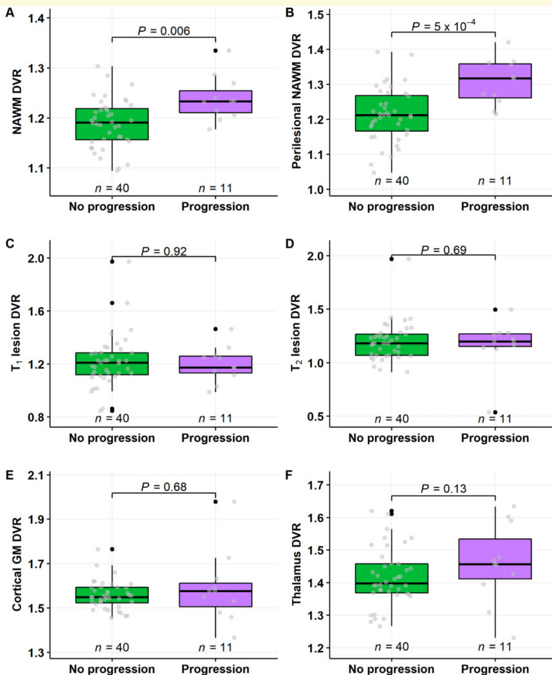
Figure 3 ^{11}\text{C} -PK11195 DVR values in multiple sclerosis patients with no relapses and with or without progression during follow-up. Innate immune cell activation was higher both in the NAWM (A) and in the perilesional NAWM (B) in patients who experienced disease progression, compared to those who did not progress. In other regions of interest, no differences between disease progression and baseline innate immune cell activation was observed (B–F). Wilcoxon rank-sum test was used. GM = grey matter.
