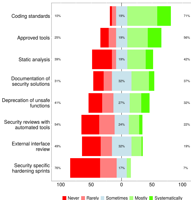
Fig. 6. Use at implementation phase.
