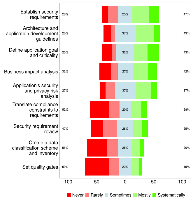
Fig. 2. Use at requirements phase.
