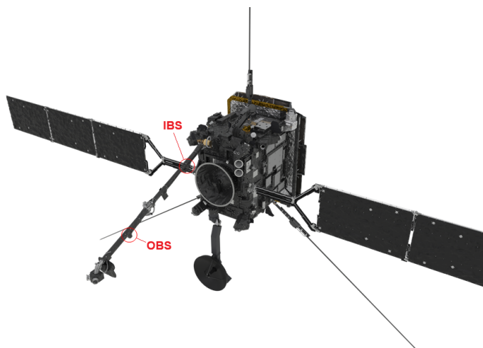
Fig. 4. The Solar Orbiter spacecraft with MAG sensors marked.
