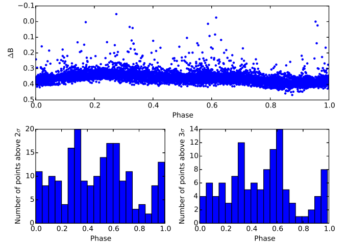
Fig. 5. Phased \Delta B light curves as used for flare statistics ( top ) and number of light curve points above 2\sigma/3\sigma after removing the effect of spottedness ( bottom ). The top plot does not show the whole magnitude range of flares to better visualise the spotted light curve.
