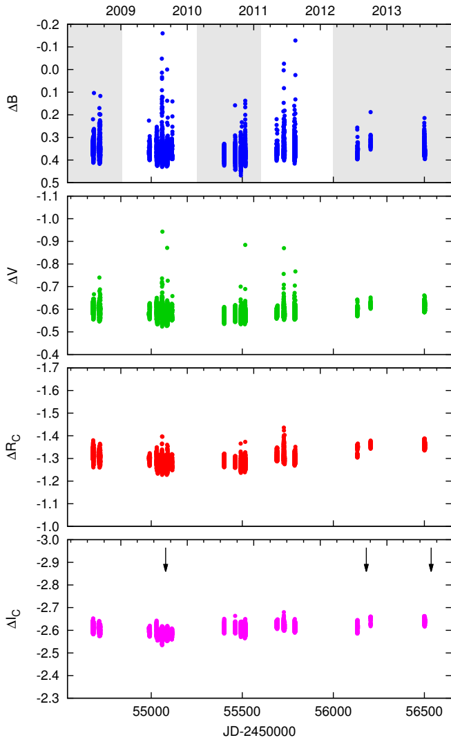
Fig. 1. BV(RI)_C photometry of V374 Peg from the Pizskéstető observations. Ranges marked in the \Delta B light curve were used for flare statistics (see Sect. 4.1). Arrows over the \Delta I light curve point at the dates of the spectroscopic observations during this time.
