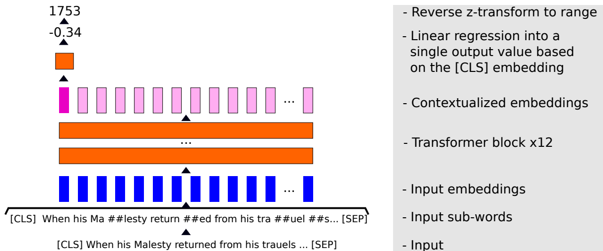
Figure 1: The regression model for a single text segment of BERT maximum sequence length, with OCR errors. Predictions across segments of a single document / book are averaged to give a final document-level prediction.
