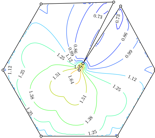
Figure 3. Contour plot of the quotient \delta_G(x, y)/\rho_G(x, y) , when G is the polygon with vertices 1, e^{0.95\pi/3}, e^{1.05\pi/3}, e^{1.05\pi/3}, e^{2\pi/3}, e^{\pi i}, e^{4\pi/3}, e^{5\pi/3} , the point x is fixed as 0 , and y varies inside G .
