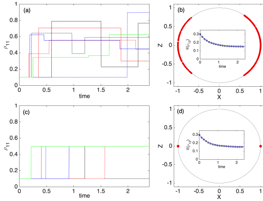
Figure 1: Simulation results using rate operator \mathbf{R1} [(a), (b)] and \mathbf{R2} [(c), (d)] for model (48) without driving. Example trajectories are displayed in (a) and (c). Final steady state distributions for Bloch vector X and Z components are shown in (b) and (d). The insets in (b) and (d) demonstrate the agreement between the analytical results (solid line) and simulation results (dots) with 10^4 trajectories. The error bars are similar to the size of the dots.
